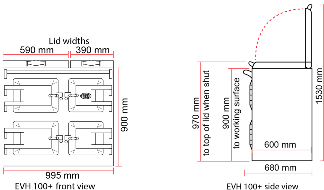
EVH100+ dimensions
