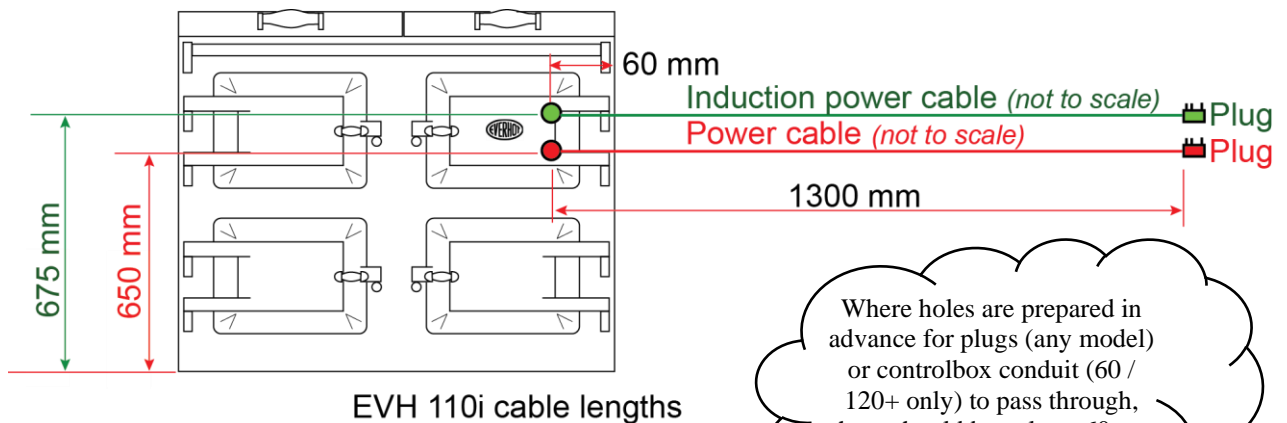
EVH110i dimensions
