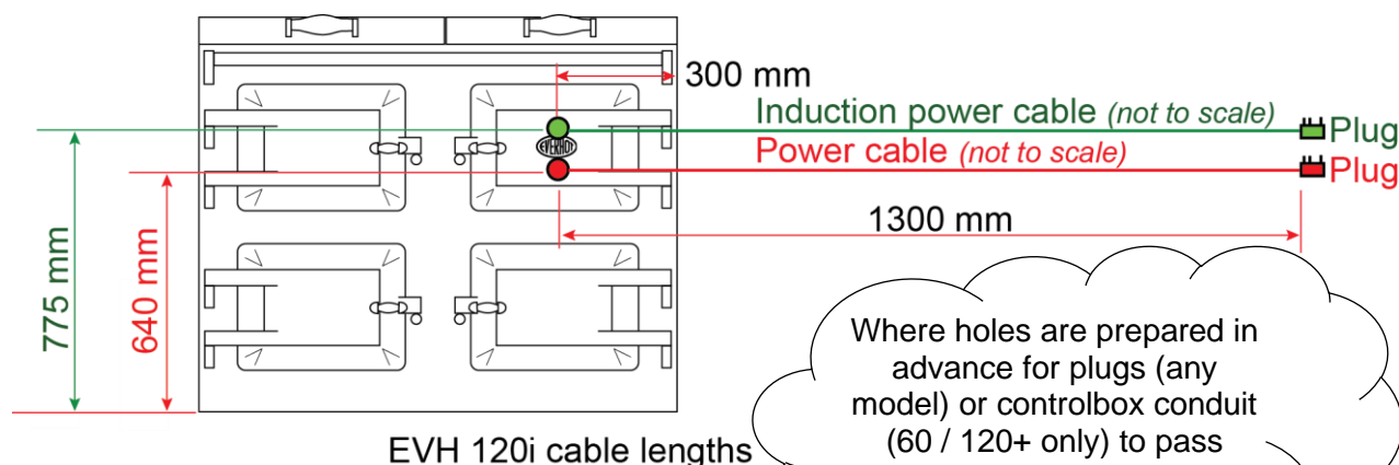
EVH120i dimensions
