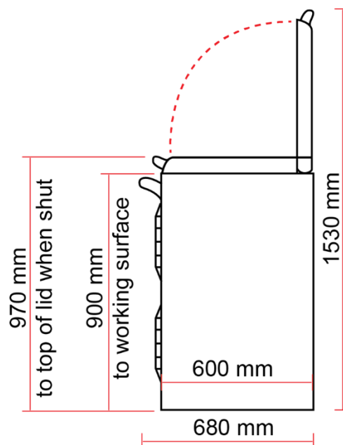
EVH 150+ side view
