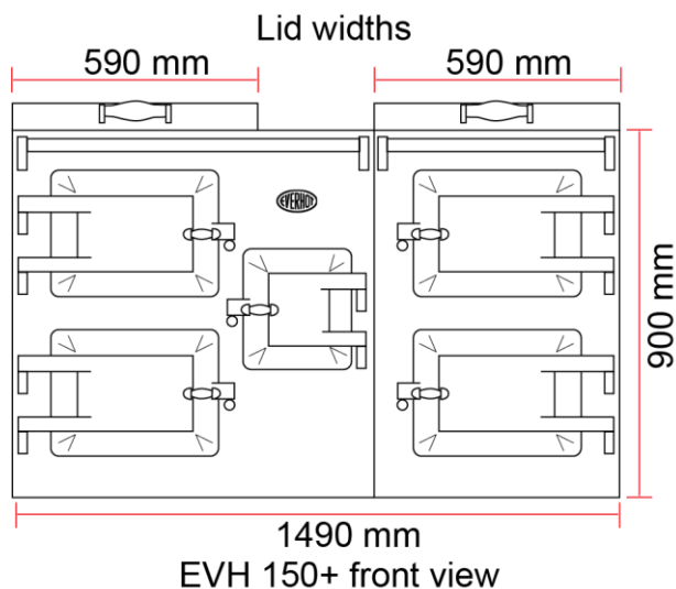
EVH150+ dimensions
