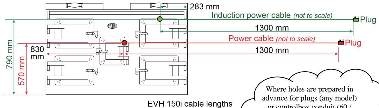
EVH150i dimensions
