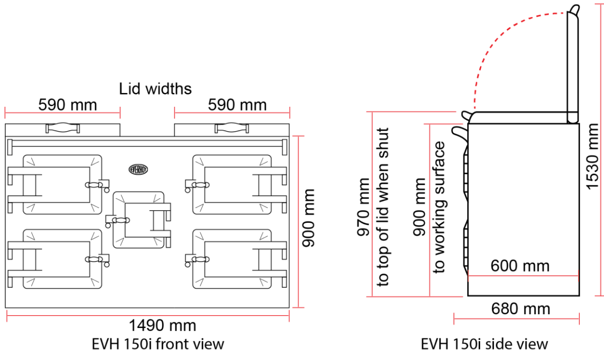
EVH150i dimensions
