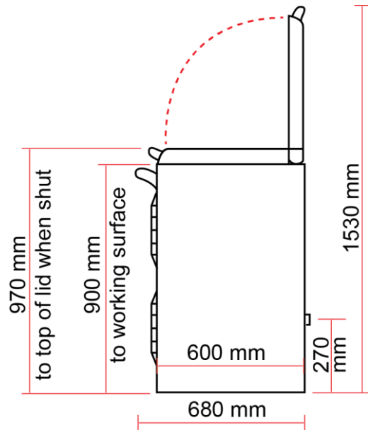
EVH 60 side view
